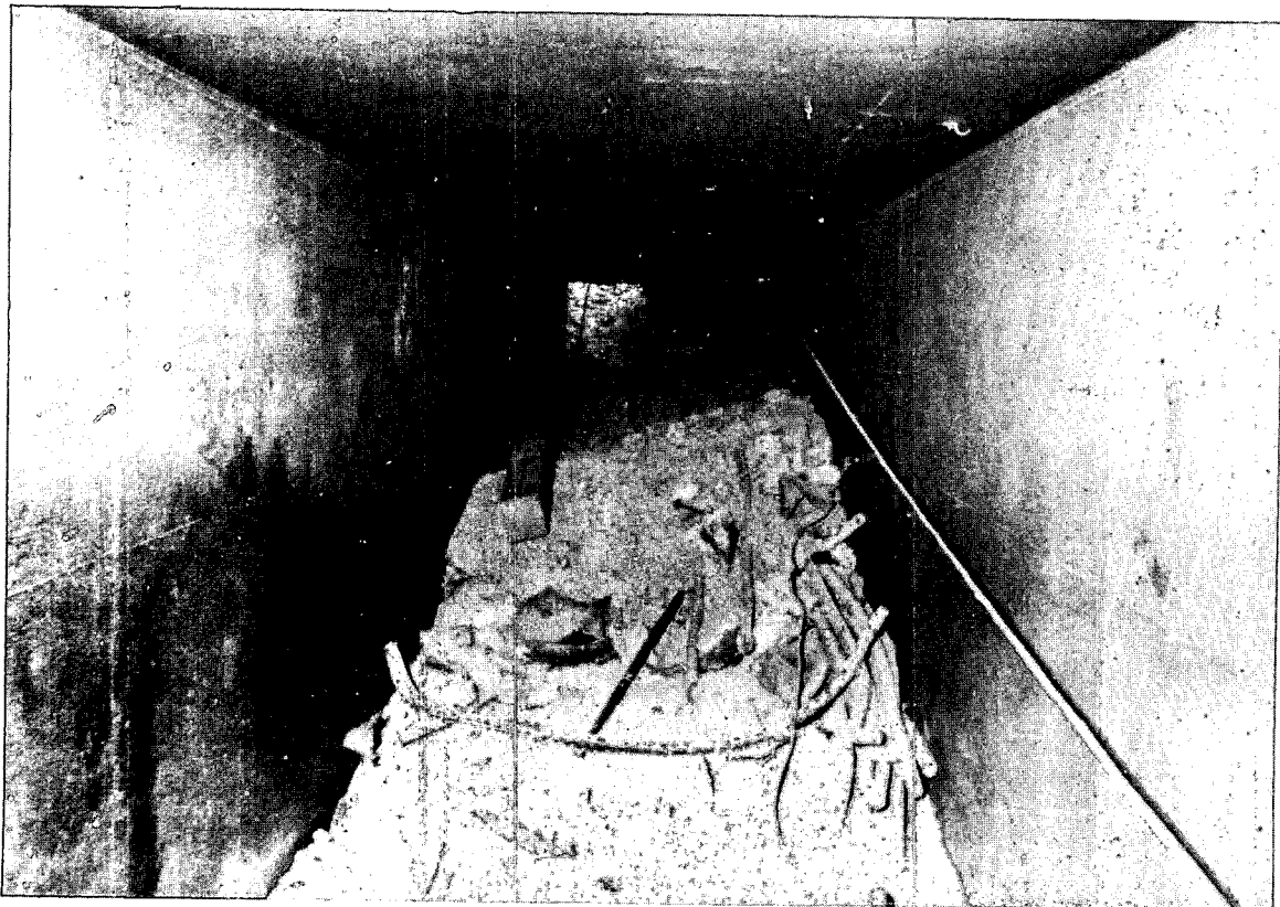
Fig. 9—Post-Quay event damage to tower-base tunnel.
